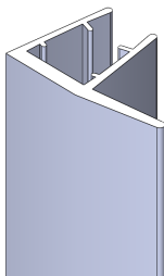
Edge seal 1x1973mm (door) 1x1910mm (fixed panel)
